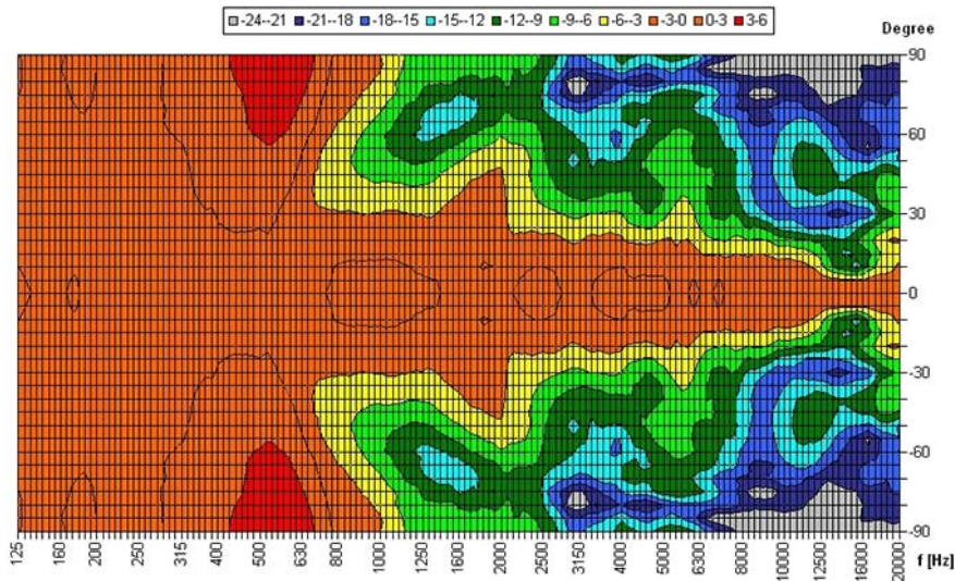
Horizontal Isobars
